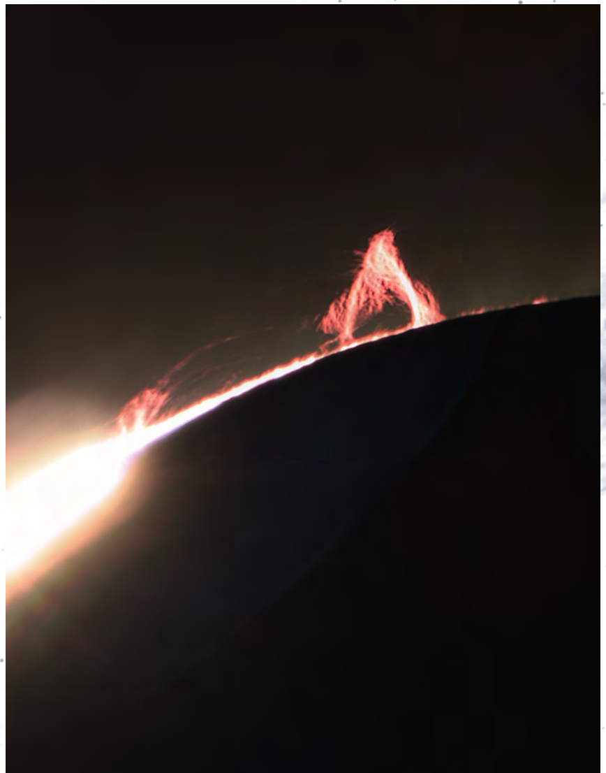
Figure 4 — This spectacular image shows two solar prominences during April's total solar eclipse. Taras Rabarskyi took this from Parc de la Gorge de Coaticook, Québec, using an 8" Meade SCT on a Celestron AVX mount with a TouCam IMX178-based camera as a roughly 7-second-long video, frames of 3096 x 2080 were aligned later in PIPP, stacked and processed in Registax with final touches done in Photoshop.
