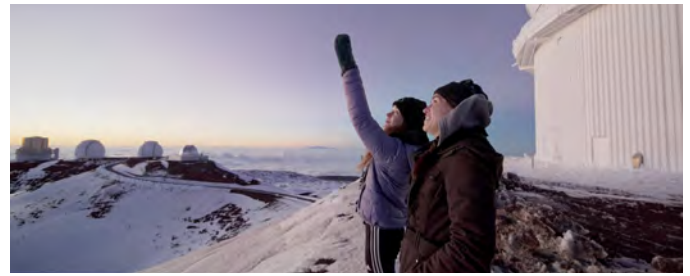
Figure 1 — Professor Laurie Rousseau-Nepton (right) and intern Justine Giroux at the Canada-France-Hawaii Telescope, where she was a Resident Astronomer, before becoming a faculty member in Astronomy and Astrophysics at the University of Toronto. Source: National Film Board of Canada.
