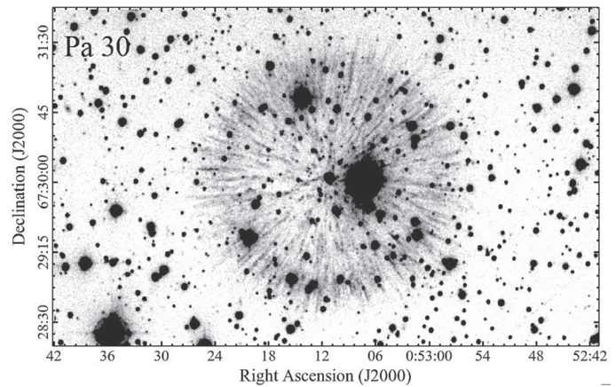
Figure 2 — An SII image of Pa 30 revealing a highly filamentary and radial morphology. Image: Robert A. Fesen, Bradley E. Schaefer, and Dana Patchick (Robert A. Fesen et al 2023 ApJL 945 L4).
