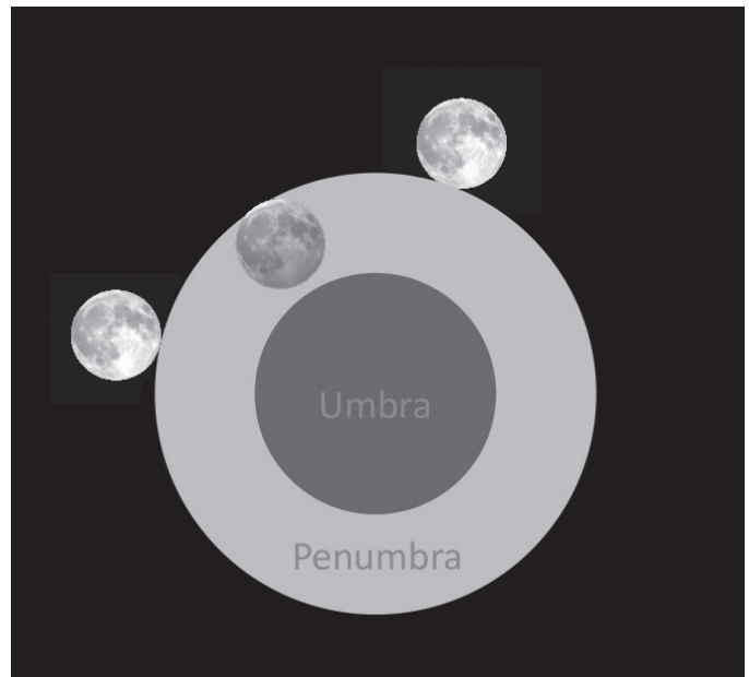
Penumbral lunar eclipse of 2024 March 25
