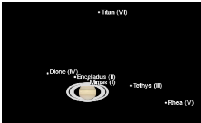
Figure 2 — The arrangement of the satellites of Saturn, 1856 April 18 at 21:15 LMT. North is up and east is on the left. The magnitudes of the satellites are: (I, 13.0), (II, 11.9), (III, 10.4), (IV, 10.5), (V, 9.8), (VI, 7.6). Smallwood likely saw the last five, Mimas being too faint. The orientation of the planet is not realistic in this Sky View Café image.
