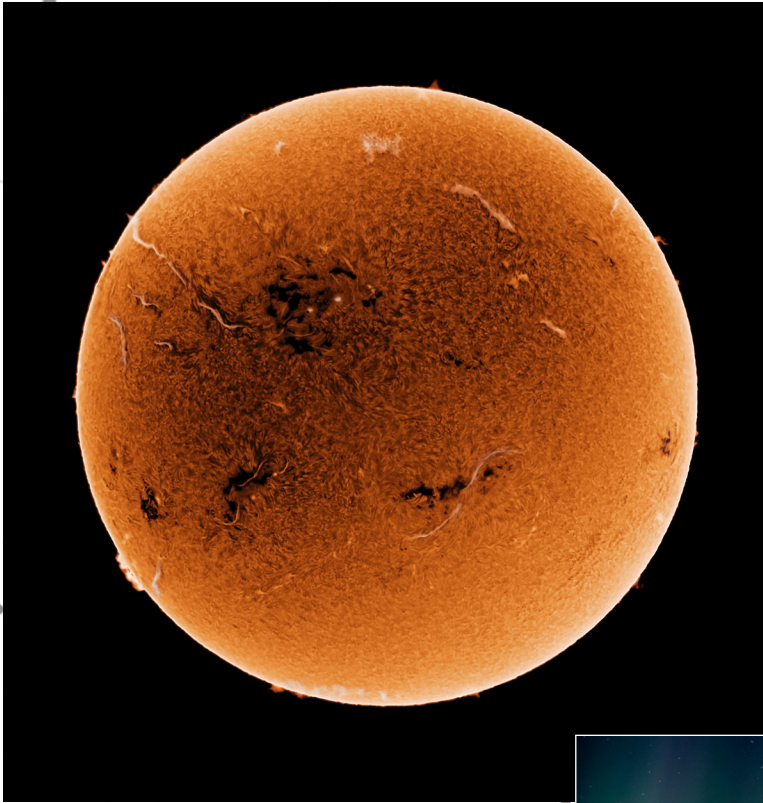
Figure 3 – Who doesn't love a spectacular image of our Sun? Shelley Jackson used a Lunt 60-mm pressure tuned H \alpha solar telescope, LS50FHa Front Mount, 50-mm DoubleStack solar filter, with a Player One Mars mono camera on a Meade 10" SCT and an LX200 mount. "The number of filaments and sunspots that day were amazing," she says. "The surface detail was spectacular. Some of the filaments seemed to creep along the surface toward the limb then erupt into a prominence."
