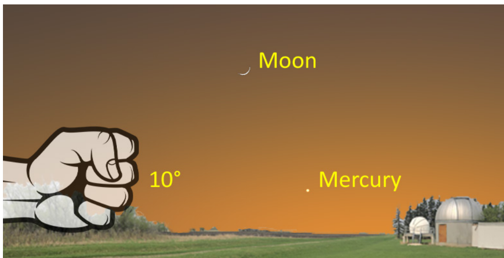
The Moon and Mercury on 2024 March 11
