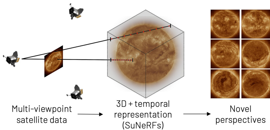
Figure 3 — A visualization of how 2-D satellite images are transformed into 3-D scenes that provide never-before-seen perspectives of the Sun. Image: NCAR & UCAR
