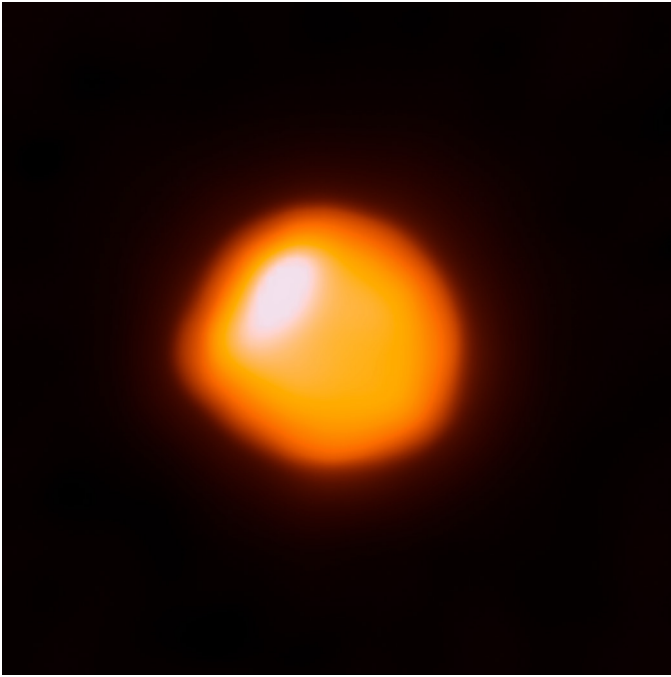
Figure 1 — ALMA image of Betelgeuse. The size of the star is comparable to the size of Jupiter's orbit and the uneven shape shows the unstable surface of the star.
