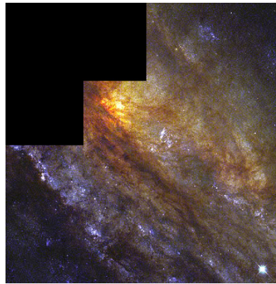
Figure 1 — NGC 253, or the Sculptor Galaxy. Credit: NASA/ESA/Hubble
