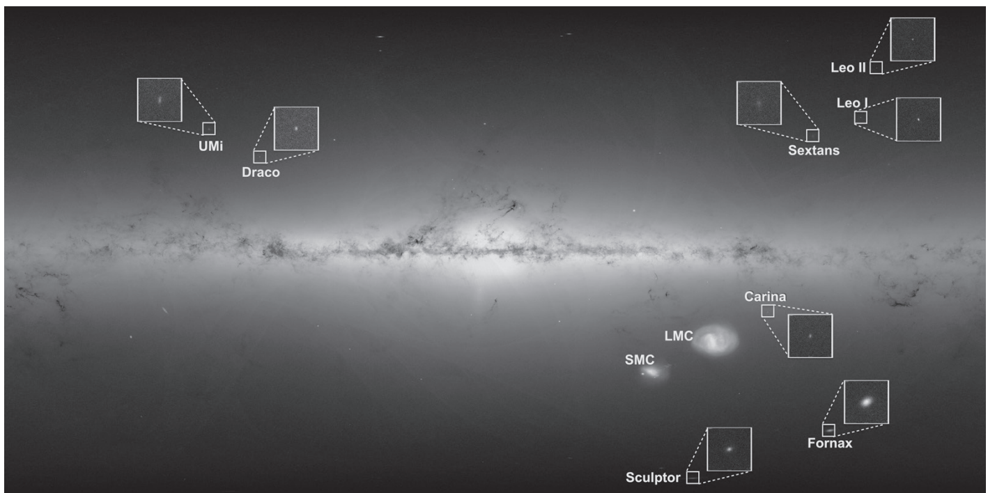
Figure 1 — Dwarf galaxies around the Milky Way. Credit: ESA/Gaia/DPAC
