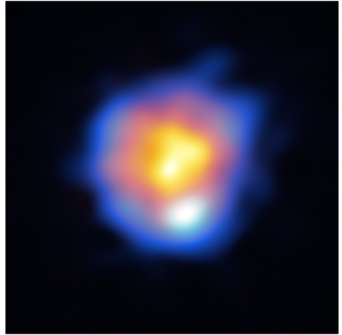
Figure 2 — ALMA image of R Leporus, an AGB star found in the constellation Lepus. The star is seen to be ejecting material in a ring around its bright surface.
