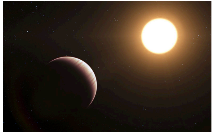
Figure 1 — Artist's rendering of Tau Boötis b and its host star. Credit: ESO/L. Calçada
