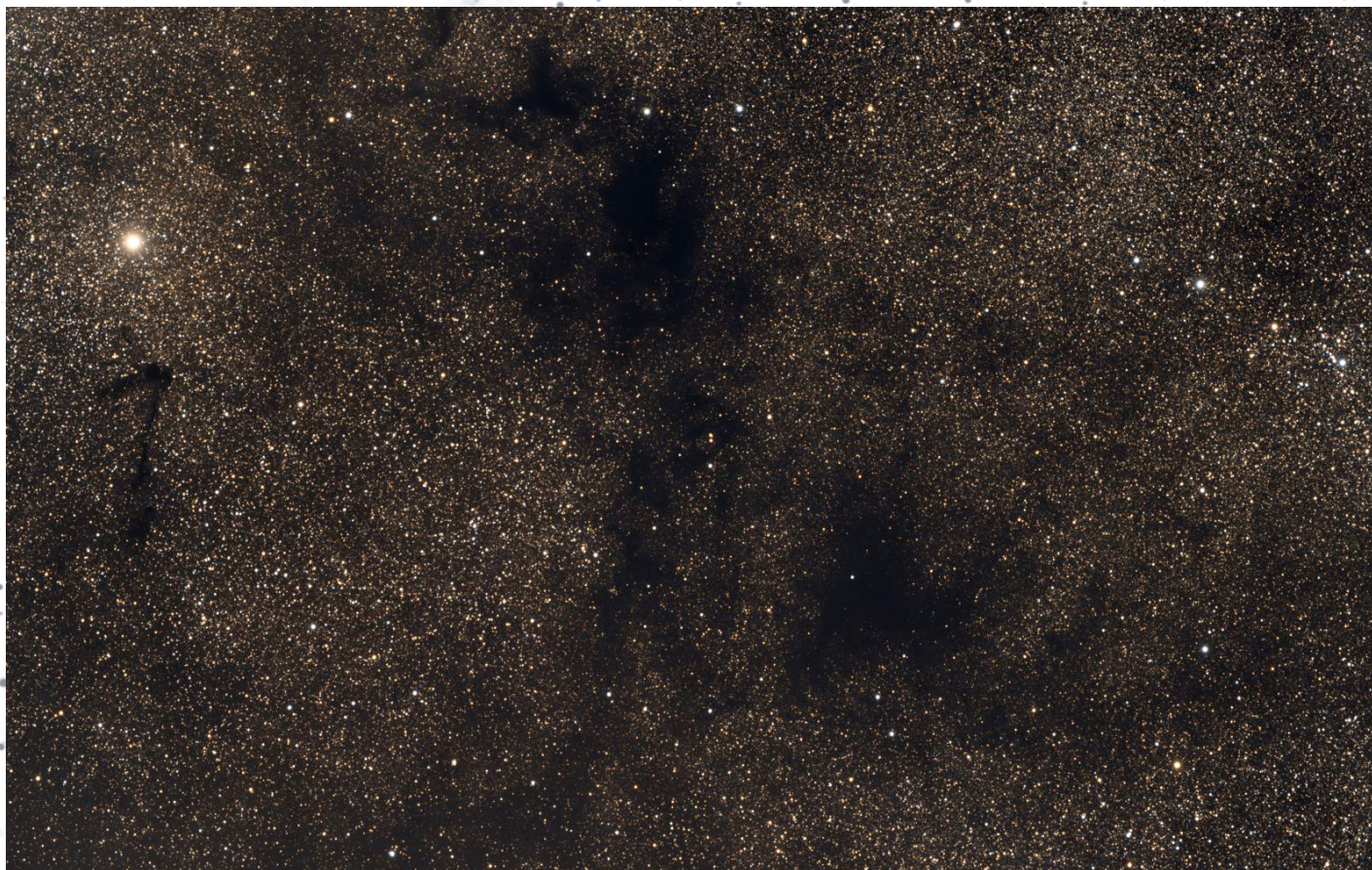
Figure 3 — Ron Brecher imaged the B110 region in Scutum, a small constellation that he describes as “overflowing with dark nebulae,” from his SkyShed in Guelph, Ontario. For luminance, he used a Sky-Watcher Esprit 150 f/7 refractor and QHY600M camera with Optolong UV/IR filter. For chrominance, he used a Takahashi FSQ-106 ED IV at f/5 and QHY367C Pro one-shot colour camera with Optolong UV/IR filter. Ron took 48 x 600-second luminance and 104 x 600-second chrominance.
