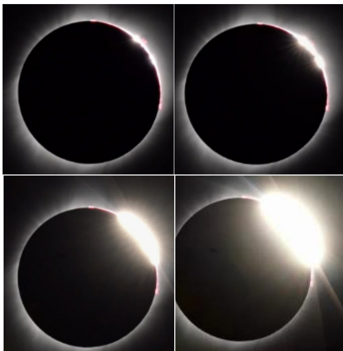
Figure 2 — Typical photos of BBs, RPs, DRs, and diffraction halos during the eclipse of 2017
