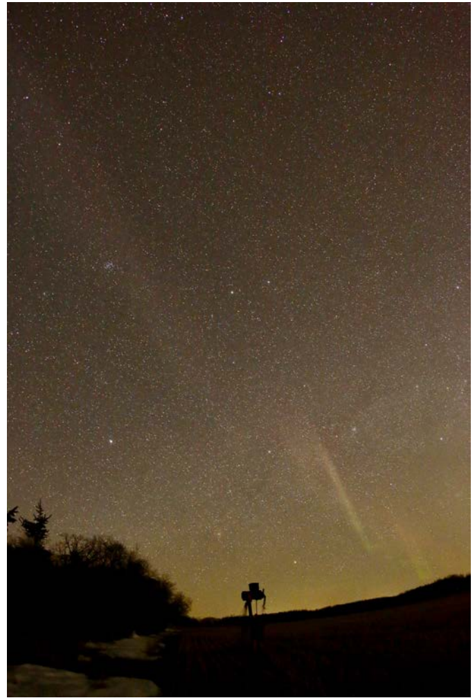
Figure 7 — In this image, acquired at 12:57 a.m., STEVE’s ribbon has almost disappeared in the eastern side (left) of the image while a few remaining banners march off toward Saskatchewan on the horizon. As in Figure 6, there is no clear separation between the green and red parts of the banners but instead a gradual transition from one colour to the other.
