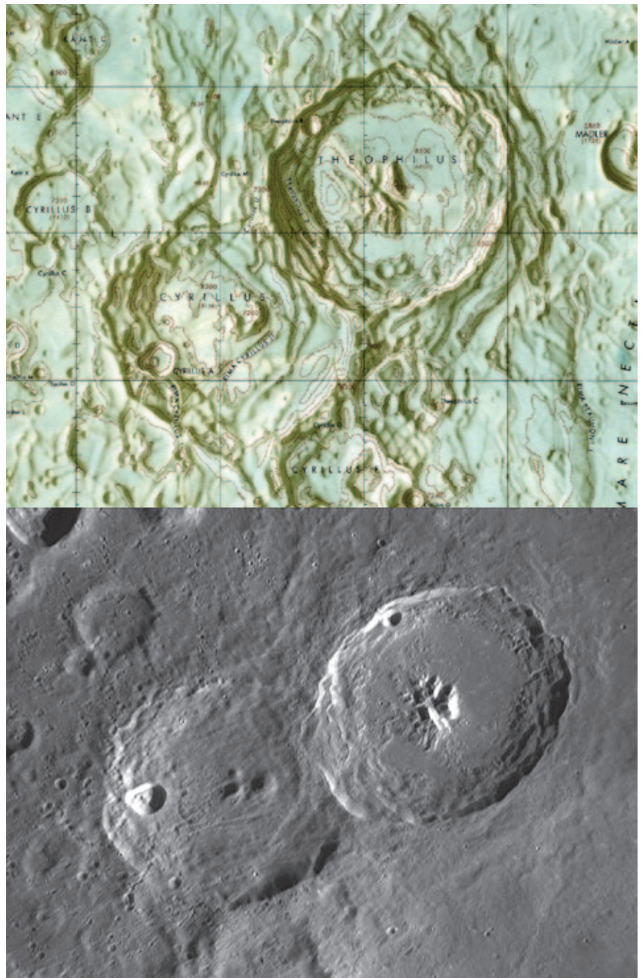
Figure 15 a,b — (top) 1963 Lunar Aeronautical Chart prepared by the United States Air Force and NASA, (bottom) amateur image captured by Leo Aerts.
