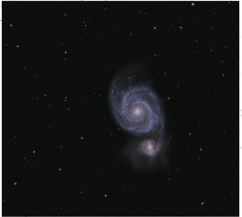
Figure 3 — Andre Paquette imaged beautiful M51 at the Barred Owl Observatory in Ottawa, Ontario. Paquette used an Apogee U16M camera on a Celestron Edge HD 14, mounted on a CGE Pro.
