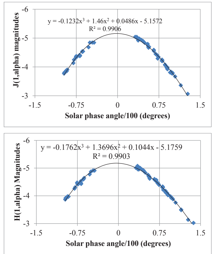
Figure 2 — J (top) and H filter (bottom) values are fitted to cubic equations according to Model 1 in Table 3. The solar phase angle, a , is the angle between the Sun and the observer measured from the centre of Venus. In the equations, y represents either J(1, a) or H(1, a) and x represents a/100 .
