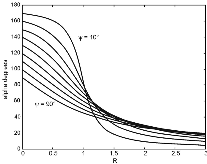
Figure 7. — The relation between \alpha , \psi and R . The graphs are drawn for \psi = 10^\circ to 90^\circ in steps of 10^\circ .
