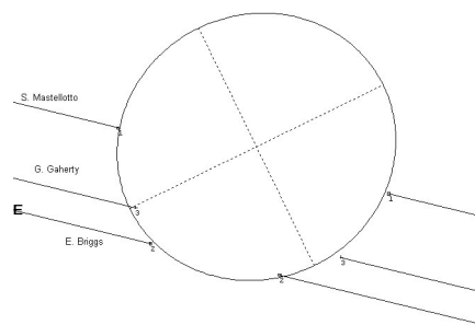
Figure 2 — Shadow outline of (31) Euphrosyne based on three occultation reports.
