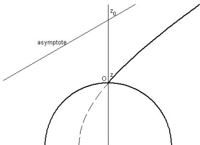
Figure 10 — Illustrating true and apparent geocentric radiants. The measured and z is the zenith distance of the apparent radiant; we need to determine the zenith distance z_0 of the true radiant.
