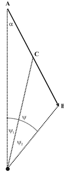
Figure 6 — The halfway point of the atmospheric trajectory does not divide the observed sky track into two equal angles.
