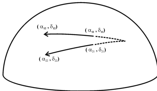
Figure 1 — Two meteors streak across the sky. The coordinates of the beginning and end of each are recorded. How do you calculate the coordinates (\alpha, \delta) of the radiant?
