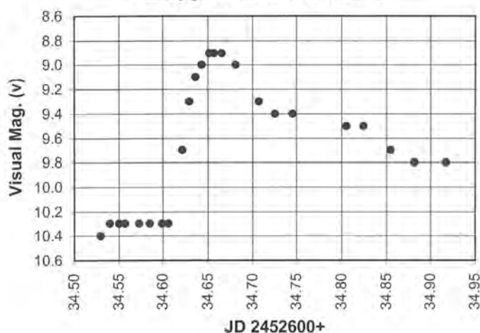
Figure 2: The visual light curve of XZ Cyg. Note the rapidity of the rise – only 53 minutes, though the exact shape of the rise is affected by the Blazhko Effect. The light curve repeats every 11.2 hours!
