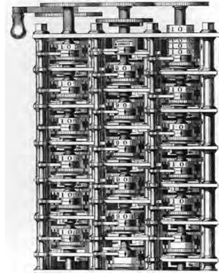
Figure 1 — While a complete Difference Engine Number 2 was never fabricated in Babbage's lifetime, a working (and programmable) arithmetic unit was assembled for its predecessor Difference Engine Number 1 in 1832. The portion constructed represented about one-seventh of the (unfinished) full-size machine, and contained nearly 2000 gears and levers (Swade, 2000). The arithmetic unit is on display next to D2 at the Science Museum in London, and it measures some 72 x 59 x 61 cm.
