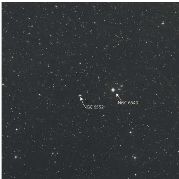
Figure 3 — 50'X50' POSS image of the field that includes NGC 6543 and NGC 6552.
